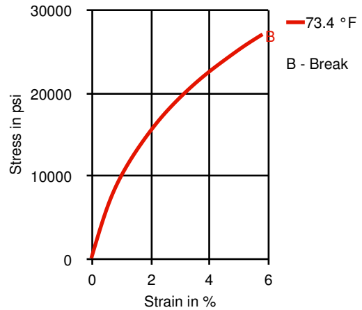
Stress-strain
